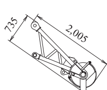
Aux. Sheave Weight: 290 kg
