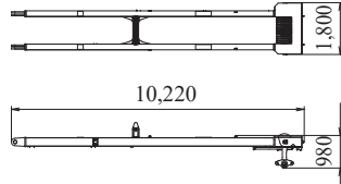
Mast Weight: 2,970 kg
