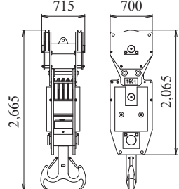
150 t Hook Weight: 2,300 kg
